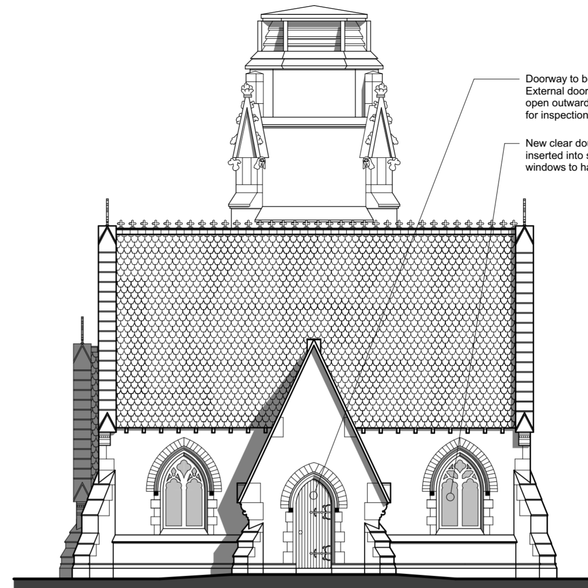
2 Proposed East Elevation Scale 1:100 @ A2
