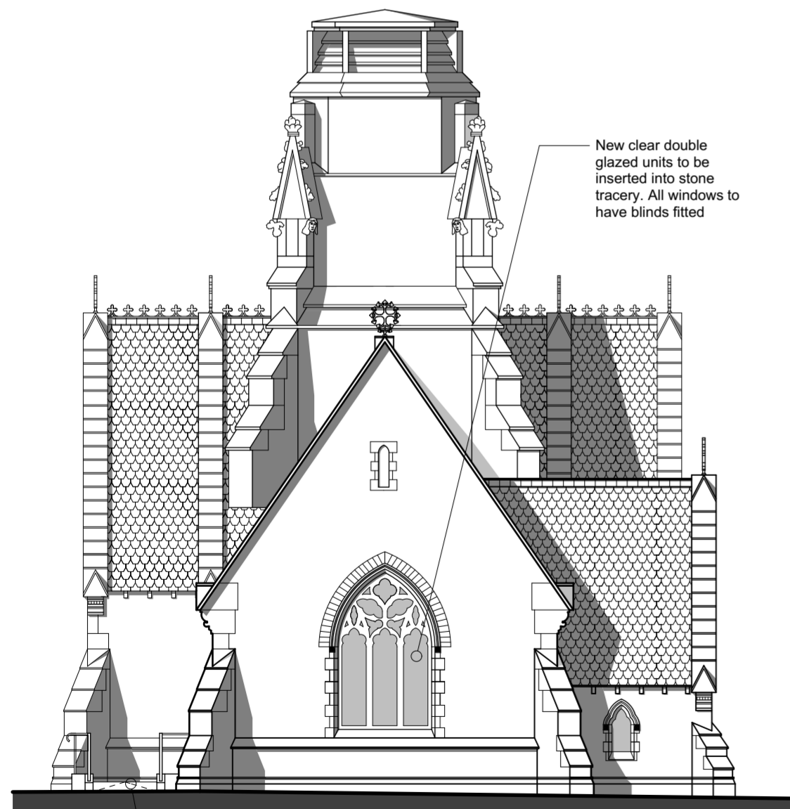
3 Proposed West Elevation Scale 1:100 @ A2
